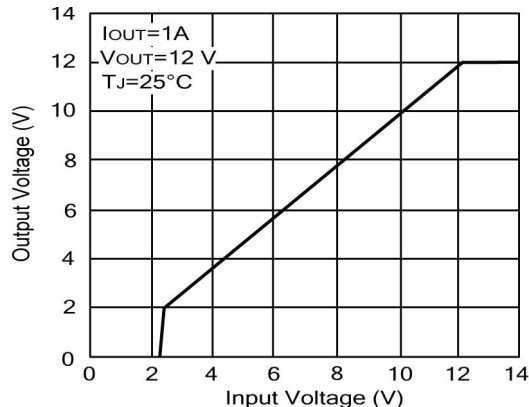
FIGURE 10. Low Voltage Behaviour
