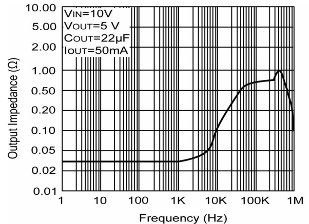
FIGURE 22. Output Impedance
