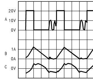
1 \mu sec/Div DS101301-18
