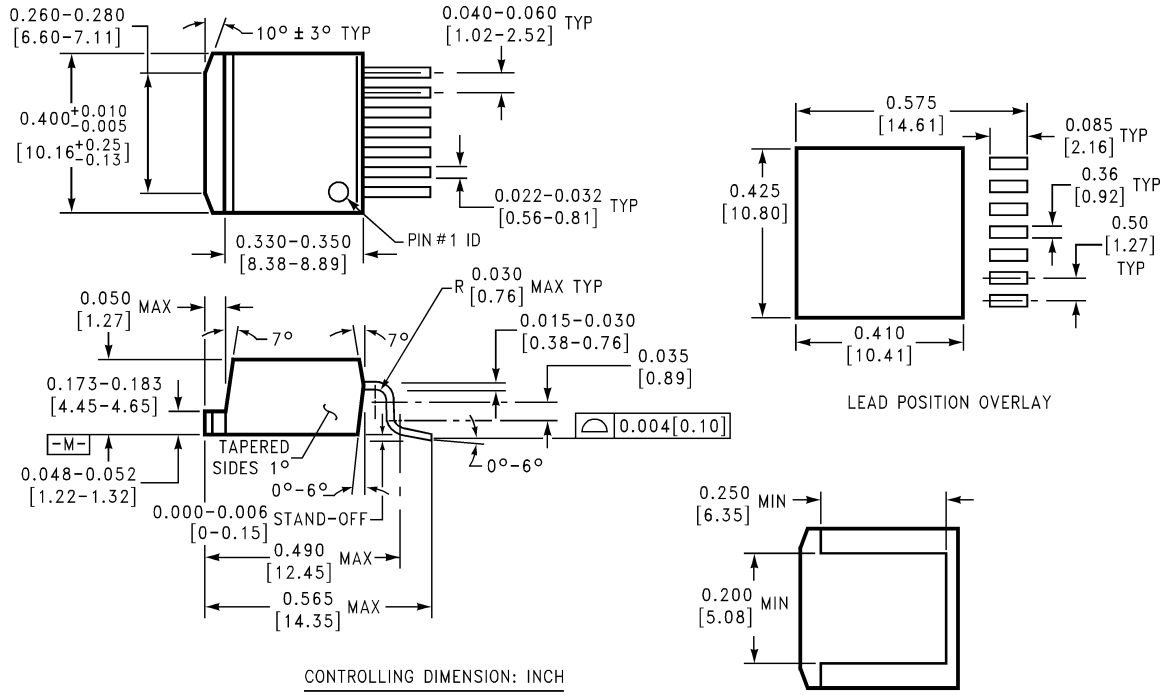
TO-263 Surface Mount Power Package Order Number LM2677S-3.3, LM2677S-5.0, LM2677S-12 or LM2677S-ADJ NS Package Number TS7B
