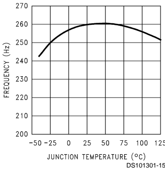
Switching Frequency
