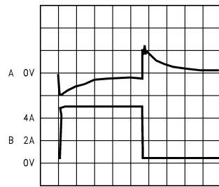
100 \mu sec/Div DS101301-19
