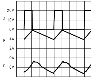
1 \mu sec/Div DS101301-17
