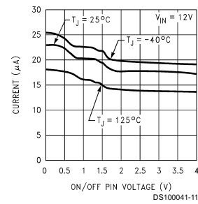
ON/OFF Pin Current (Sourcing)
