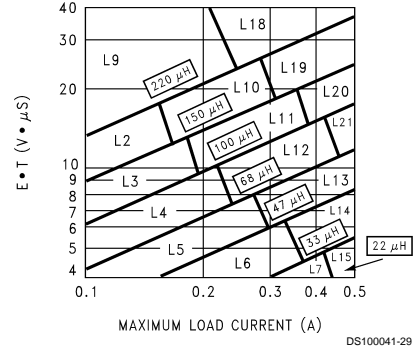
FIGURE 7. LM2674-ADJ
