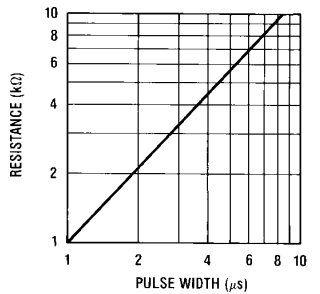
FIGURE 8. Pulse Stretcher Resistance vs Pulse Width
