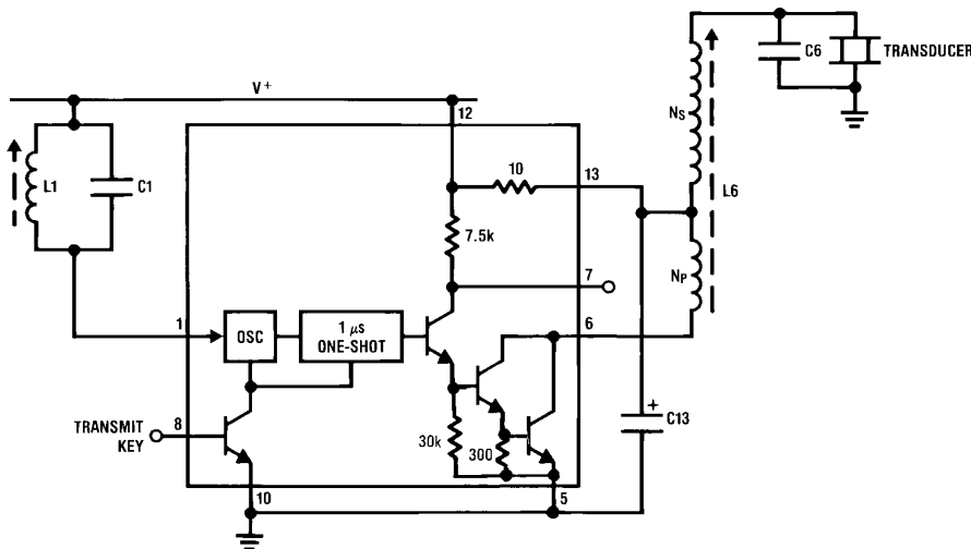
FIGURE 5. Transmitter
