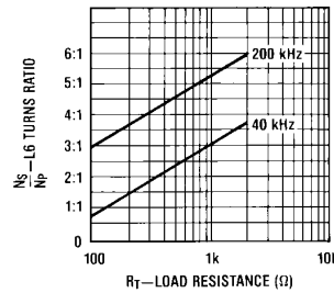
FIGURE 6. L6 Turns Ratio vs Load Resistance
