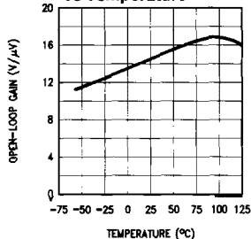
Open-Loop Gain vs Temperature
