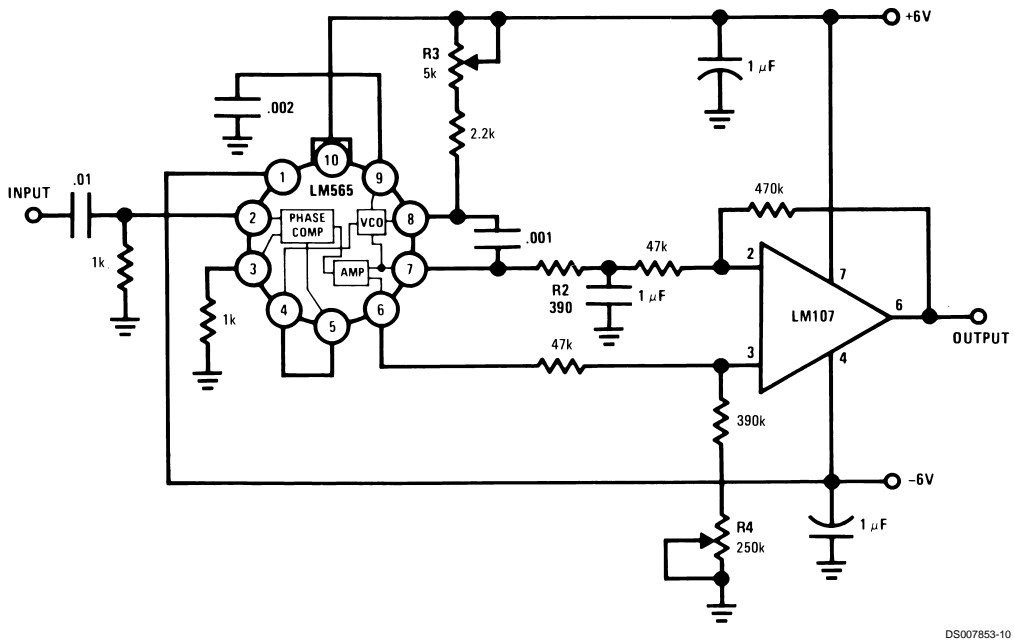
IRIG Channel 13 Demodulator
